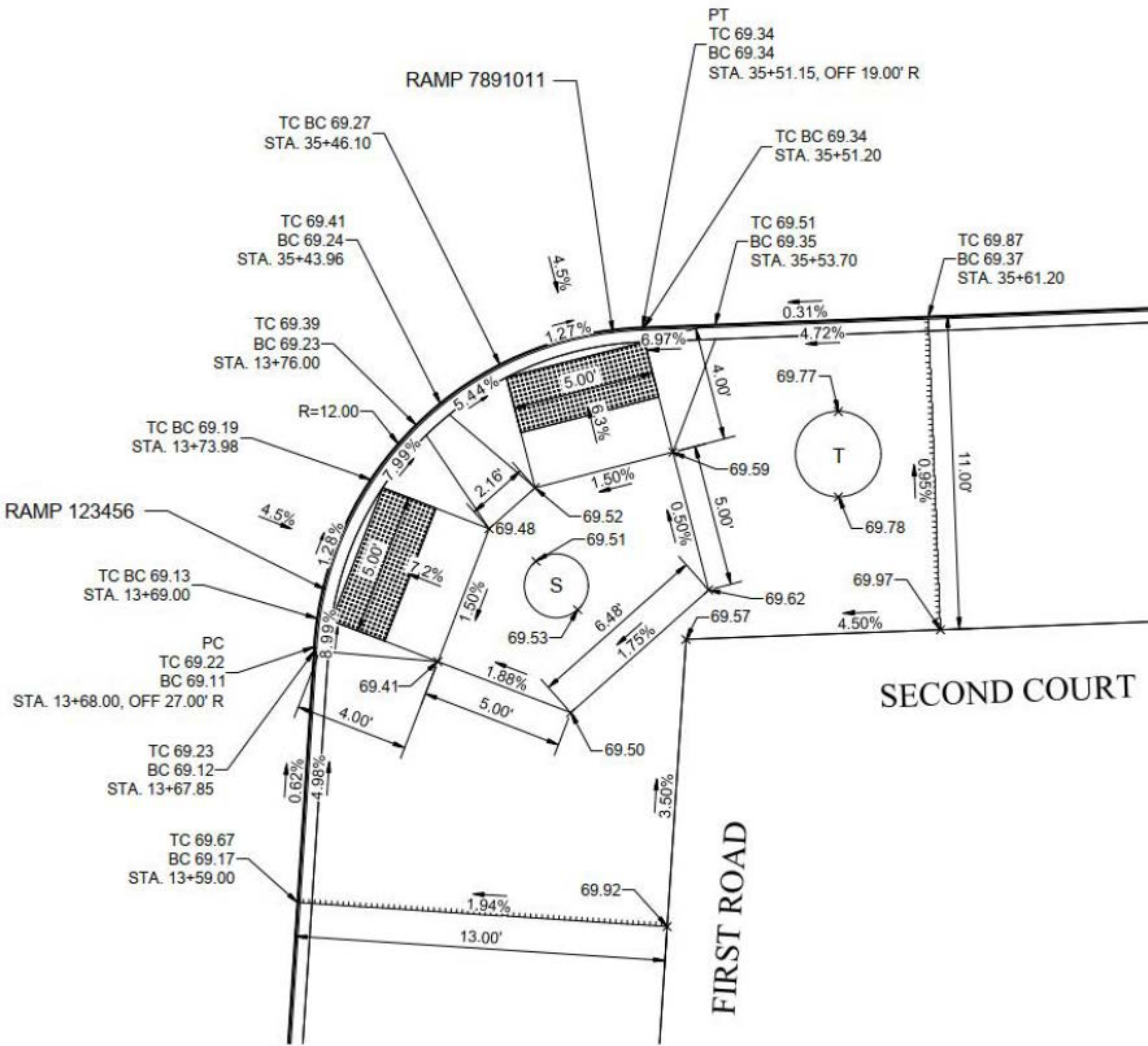
GRADING DETAIL - LOCATION X, SE CORNER
